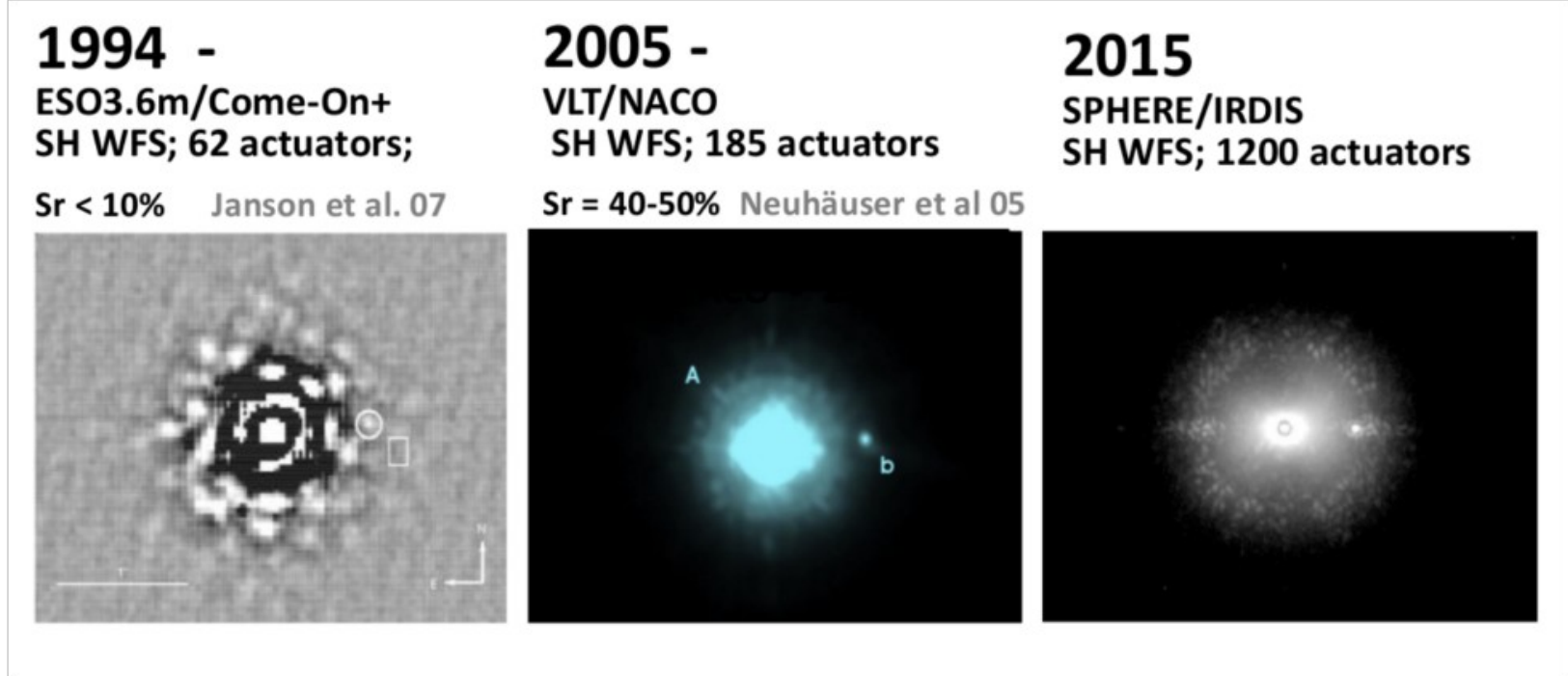
Figure 2. Observation of the young GQ Lupi star (K7V; V = 11.4 ; K = 7.1 ) hosting a brown dwarf companion located at 730 mas with three generations of ESO AO instruments: ESO3.6m/Come-On+, NaCo and SPHERE at VLT.
