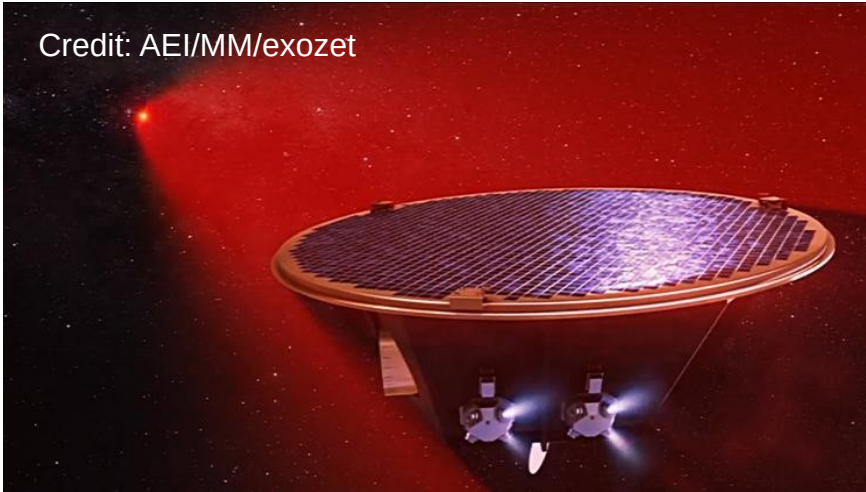
LISA
